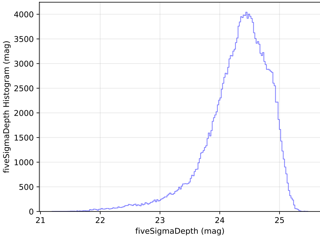
too_elab_r64_d3_giz_v3.4_10yrs WFD g band: fiveSigmaDepth Histogram
