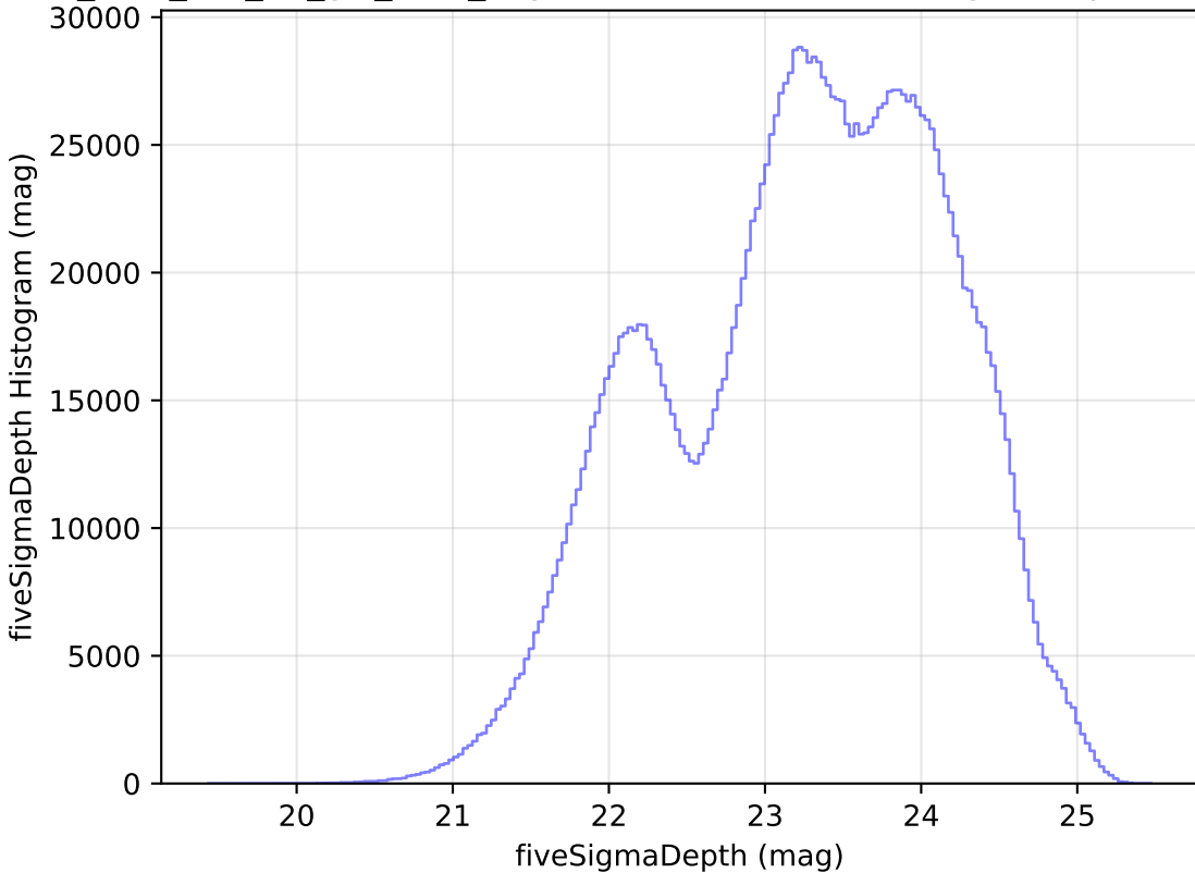
too_elab_r64_d3_giz_v3.4_10yrs WFD all bands: fiveSigmaDepth Histogram
