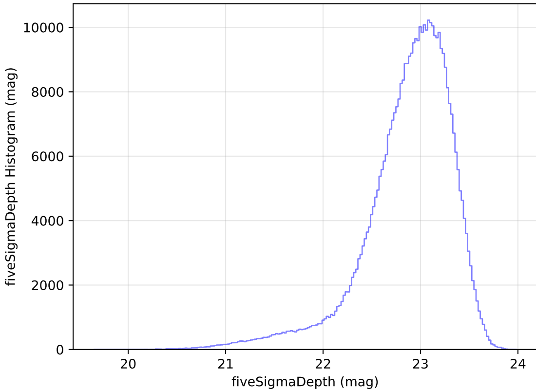
too_elab_r64_d3_giz_v3.4_10yrs All sky z band: fiveSigmaDepth Histogram
