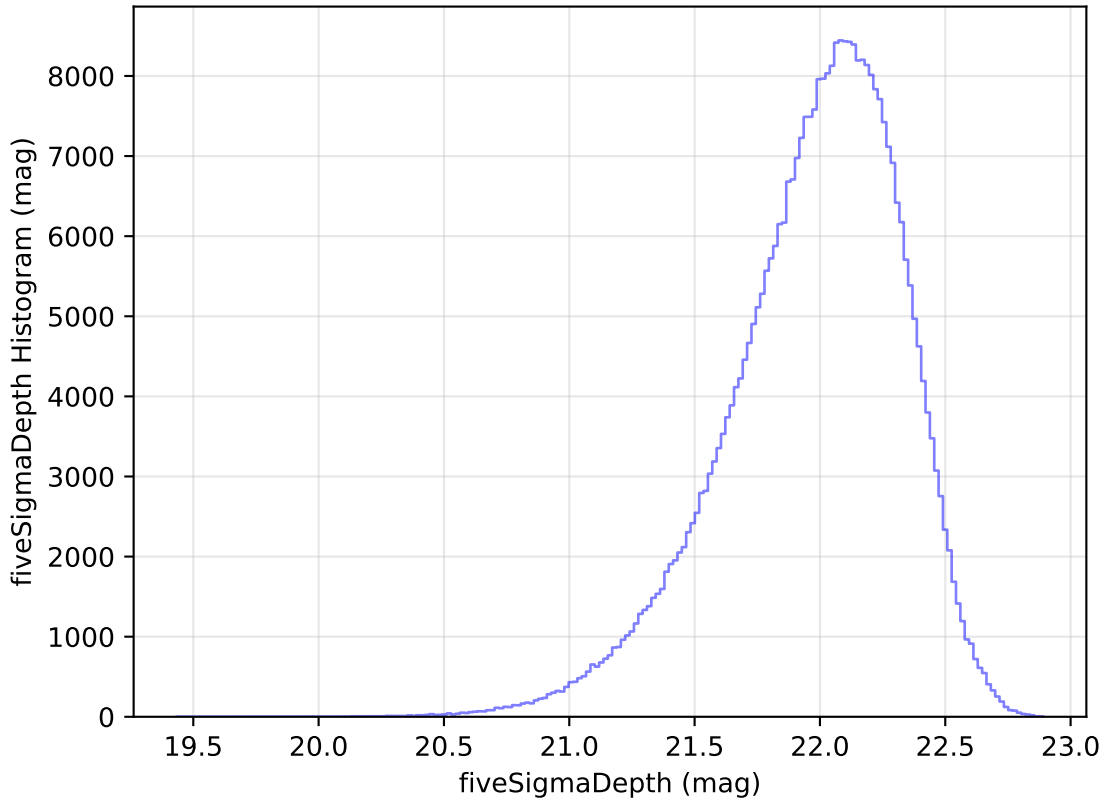
too_elab_r64_d3_giz_v3.4_10yrs All sky y band: fiveSigmaDepth Histogram
