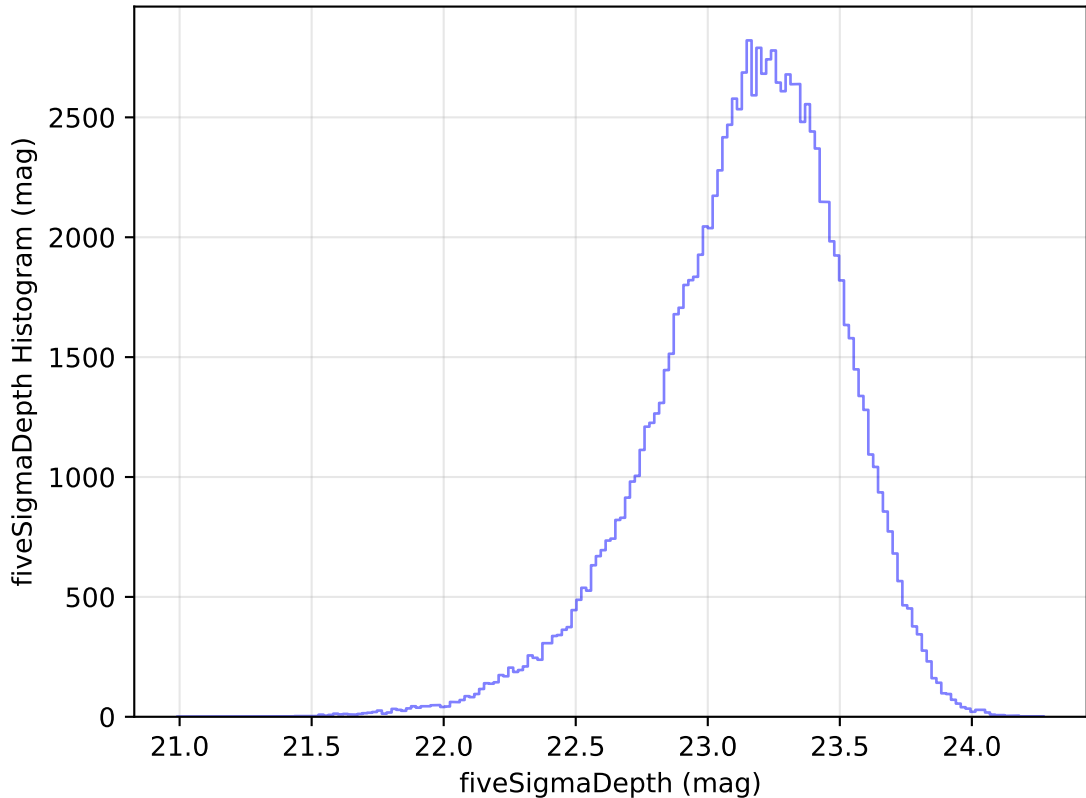
too_elab_r64_d3_giz_v3.4_10yrs All sky u band: fiveSigmaDepth Histogram
