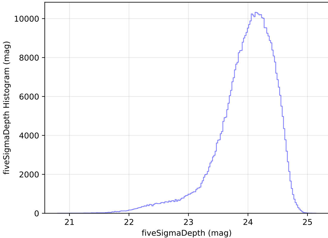
too_elab_r64_d3_giz_v3.4_10yrs All sky r band: fiveSigmaDepth Histogram
