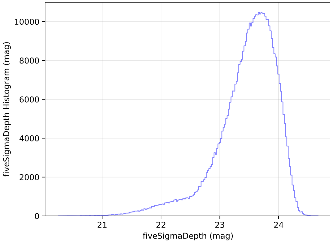
too_elab_r64_d3_giz_v3.4_10yrs All sky i band: fiveSigmaDepth Histogram
