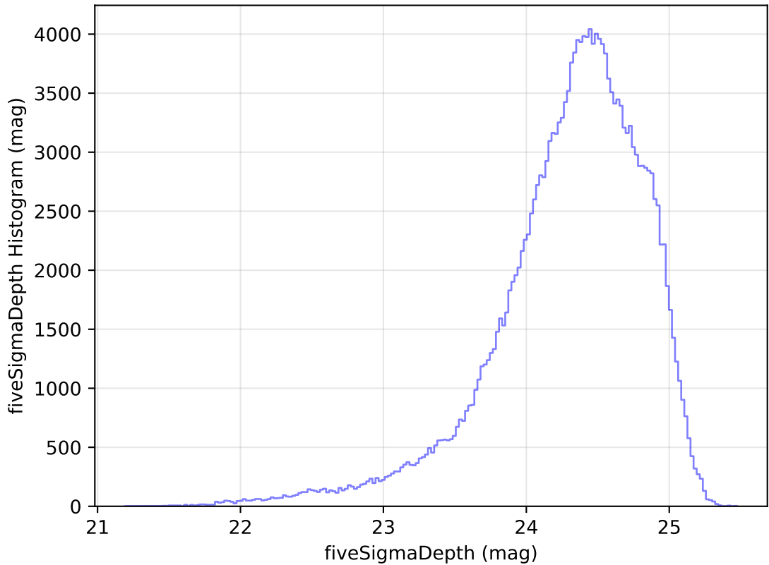
too_elab_r64_d3_giz_v3.4_10yrs All sky g band: fiveSigmaDepth Histogram
