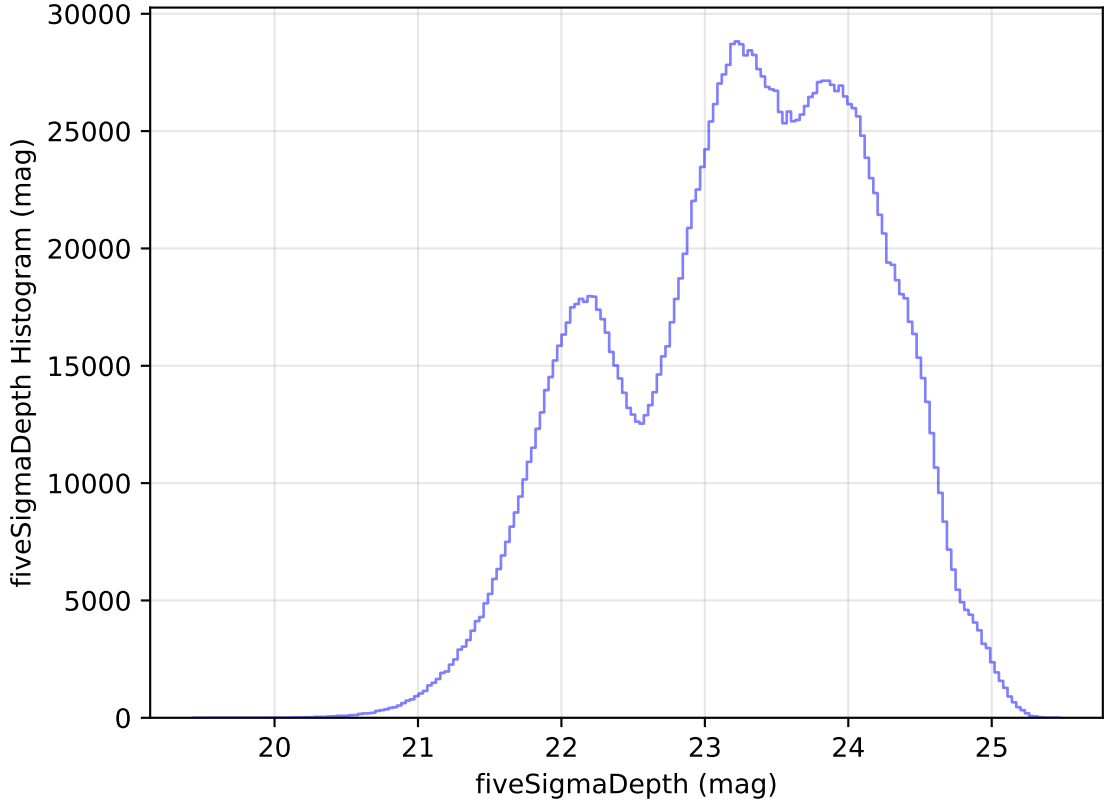
too_elab_r64_d3_giz_v3.4_10yrs All sky all bands: fiveSigmaDepth Histogram
