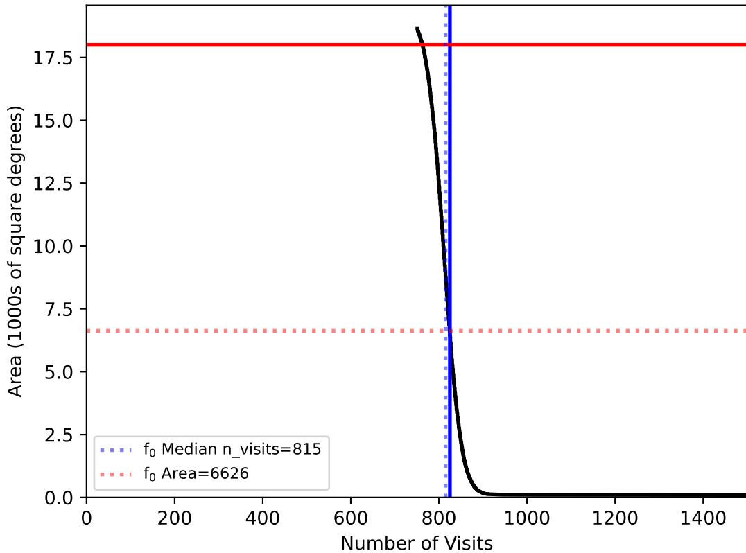
too_elab_r64_d3_giz_v3.4_10yrs WFD: f0
