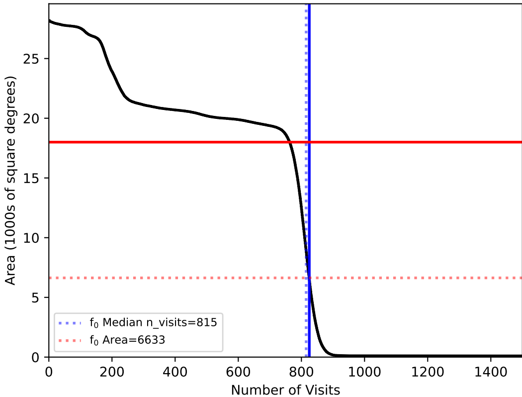
too_elab_r64_d3_giz_v3.4_10yrs All sky: f0
