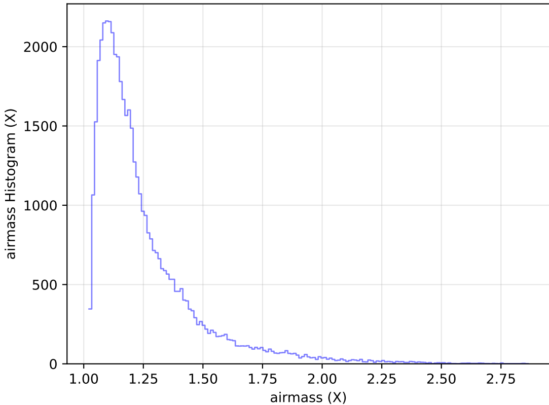
too_elab_r64_d3_giz_v3.4_10yrs Yr 1 y band: airmass Histogram
