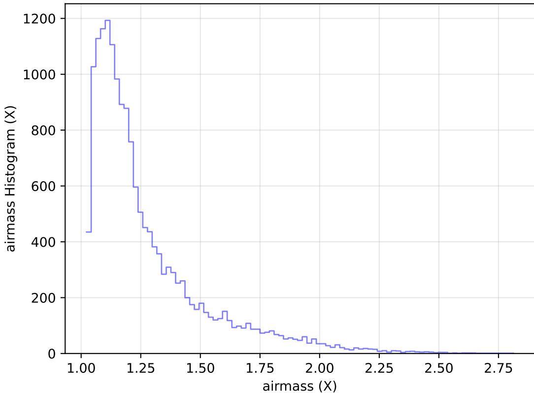
too_elab_r64_d3_giz_v3.4_10yrs Yr 1 u band: airmass Histogram
