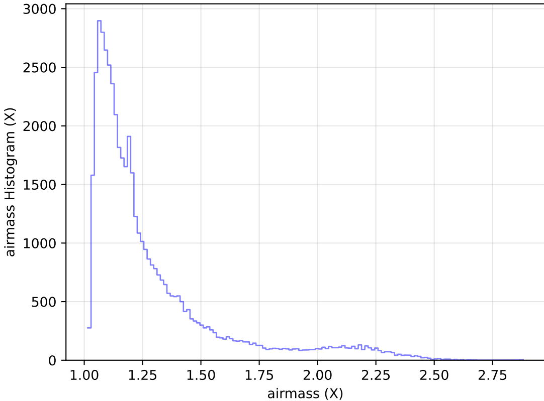
too_elab_r64_d3_giz_v3.4_10yrs Yr 1 r band: airmass Histogram
