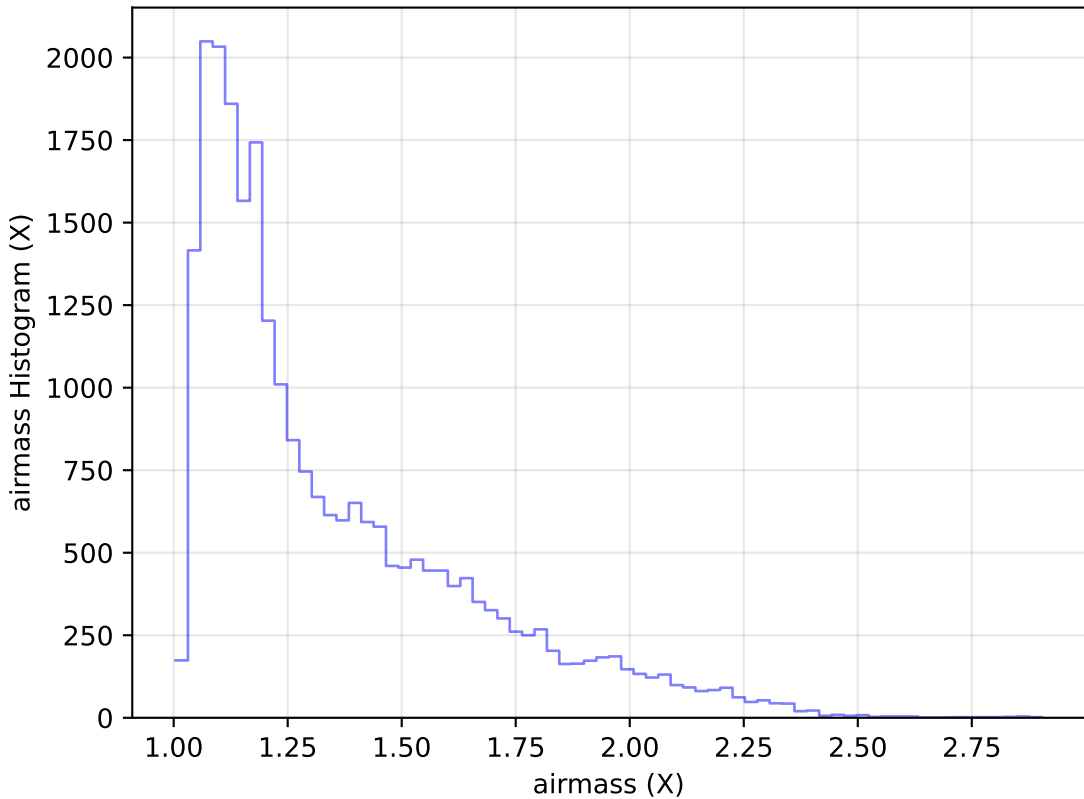
too_elab_r64_d3_giz_v3.4_10yrs Yr 1 g band: airmass Histogram
