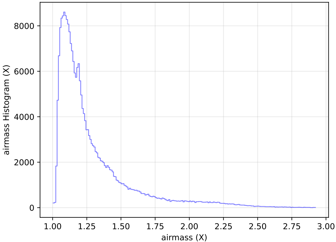
too_elab_r64_d3_giz_v3.4_10yrs Yr 1 all bands: airmass Histogram
