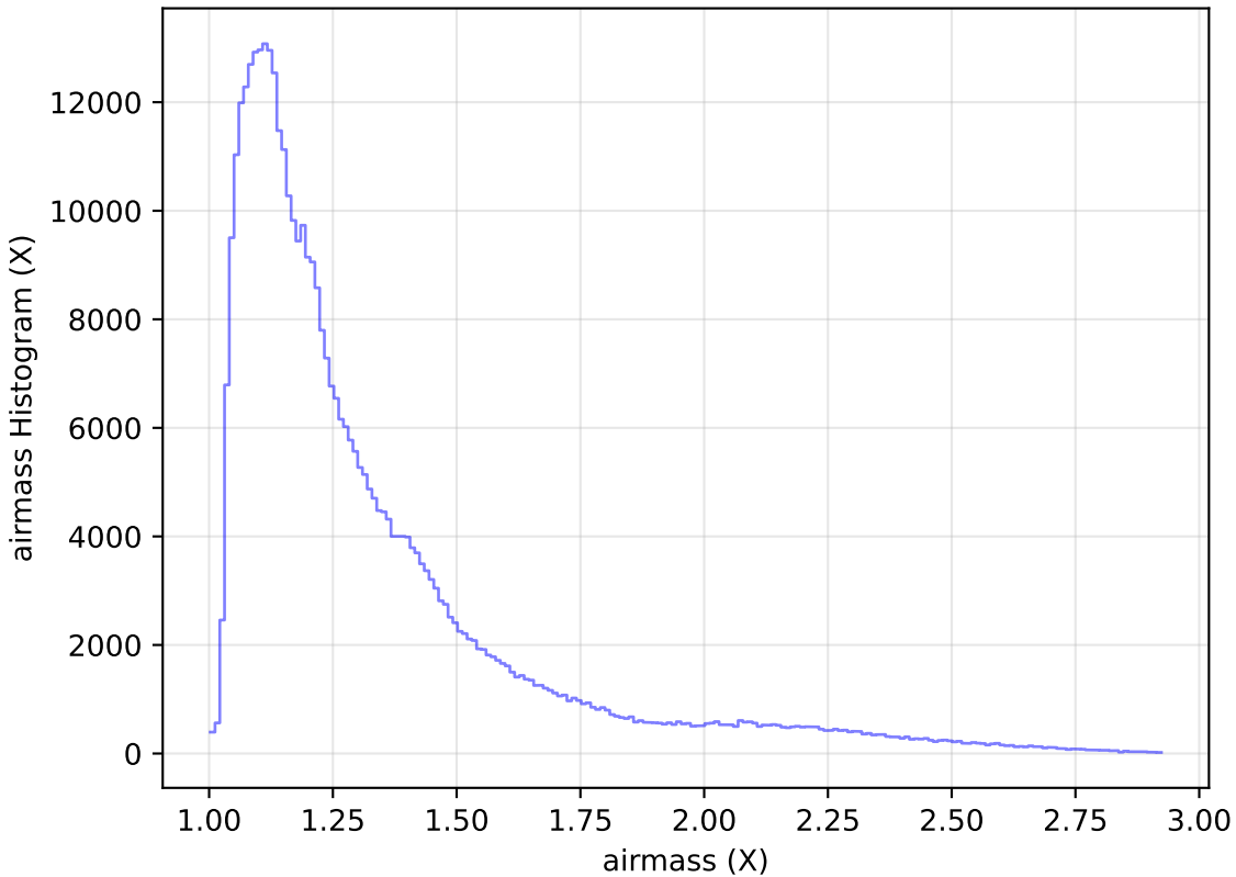
too_elab_r64_d3_giz_v3.4_10yrs WFD z band: airmass Histogram
