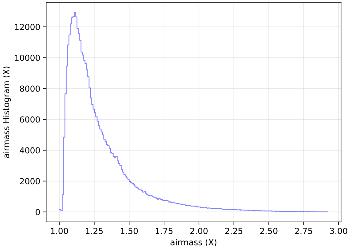
too_elab_r64_d3_giz_v3.4_10yrs WFD y band: airmass Histogram
