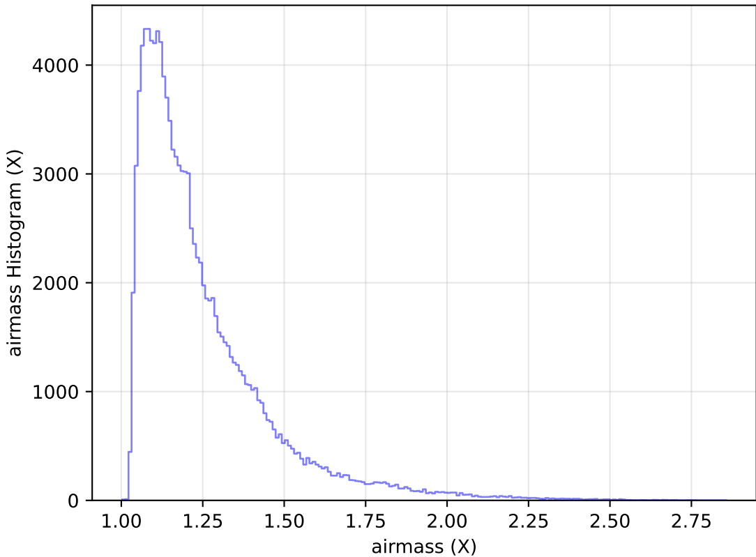
too_elab_r64_d3_giz_v3.4_10yrs WFD u band: airmass Histogram
