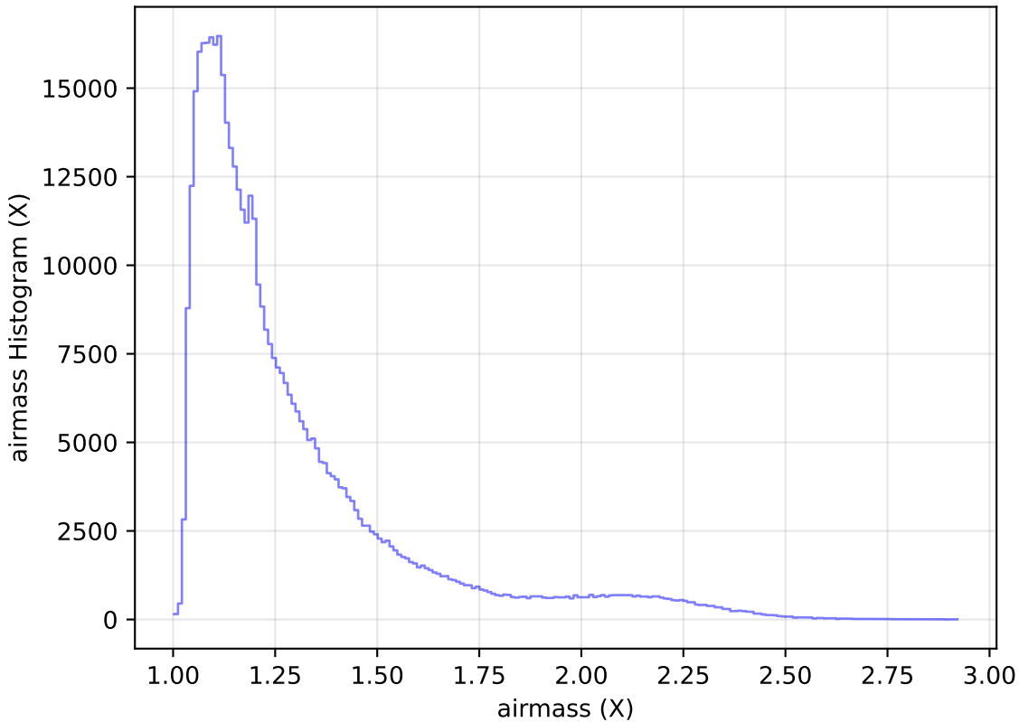
too_elab_r64_d3_giz_v3.4_10yrs WFD r band: airmass Histogram
