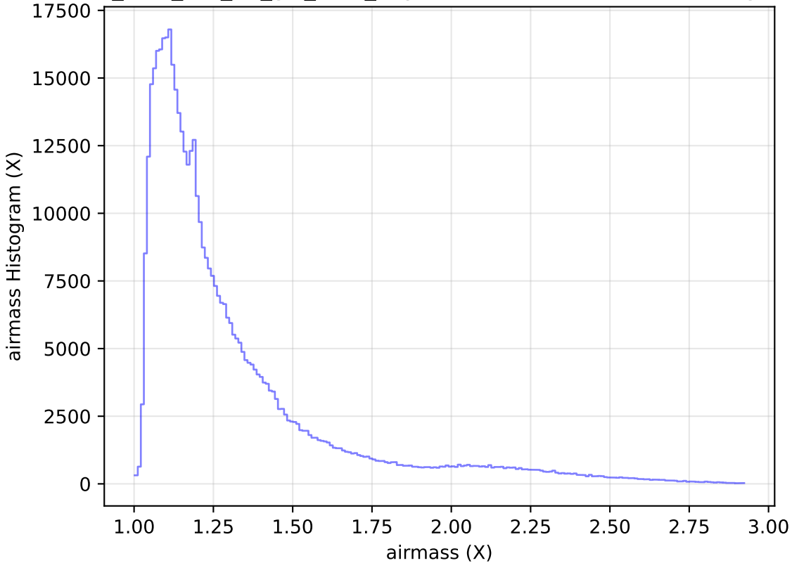
too_elab_r64_d3_giz_v3.4_10yrs WFD i band: airmass Histogram
