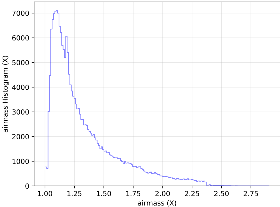
too_elab_r64_d3_giz_v3.4_10yrs WFD g band: airmass Histogram
