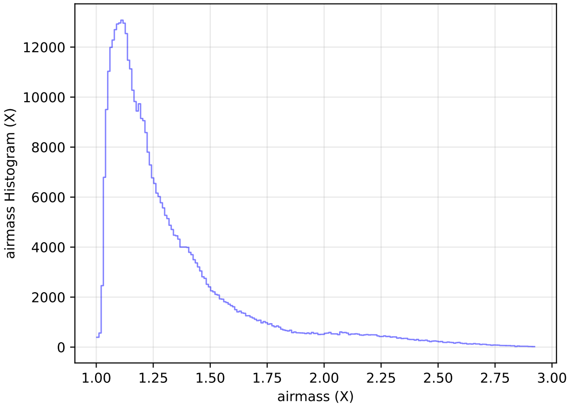
too_elab_r64_d3_giz_v3.4_10yrs All sky z band: airmass Histogram
