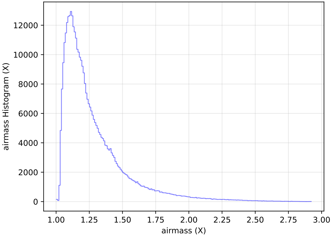
too_elab_r64_d3_giz_v3.4_10yrs All sky y band: airmass Histogram
