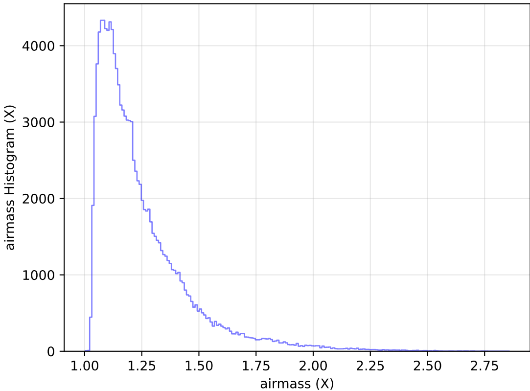
too_elab_r64_d3_giz_v3.4_10yrs All sky u band: airmass Histogram
