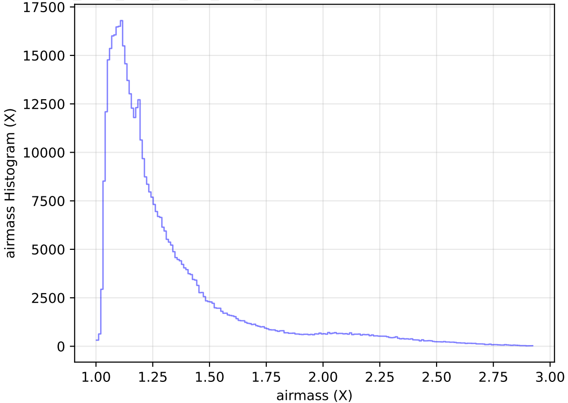
too_elab_r64_d3_giz_v3.4_10yrs All sky i band: airmass Histogram
