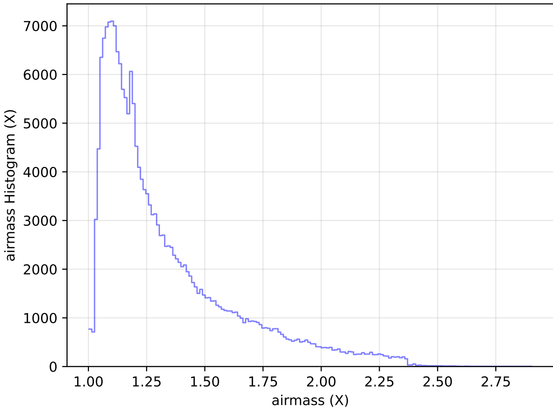
too_elab_r64_d3_giz_v3.4_10yrs All sky g band: airmass Histogram
