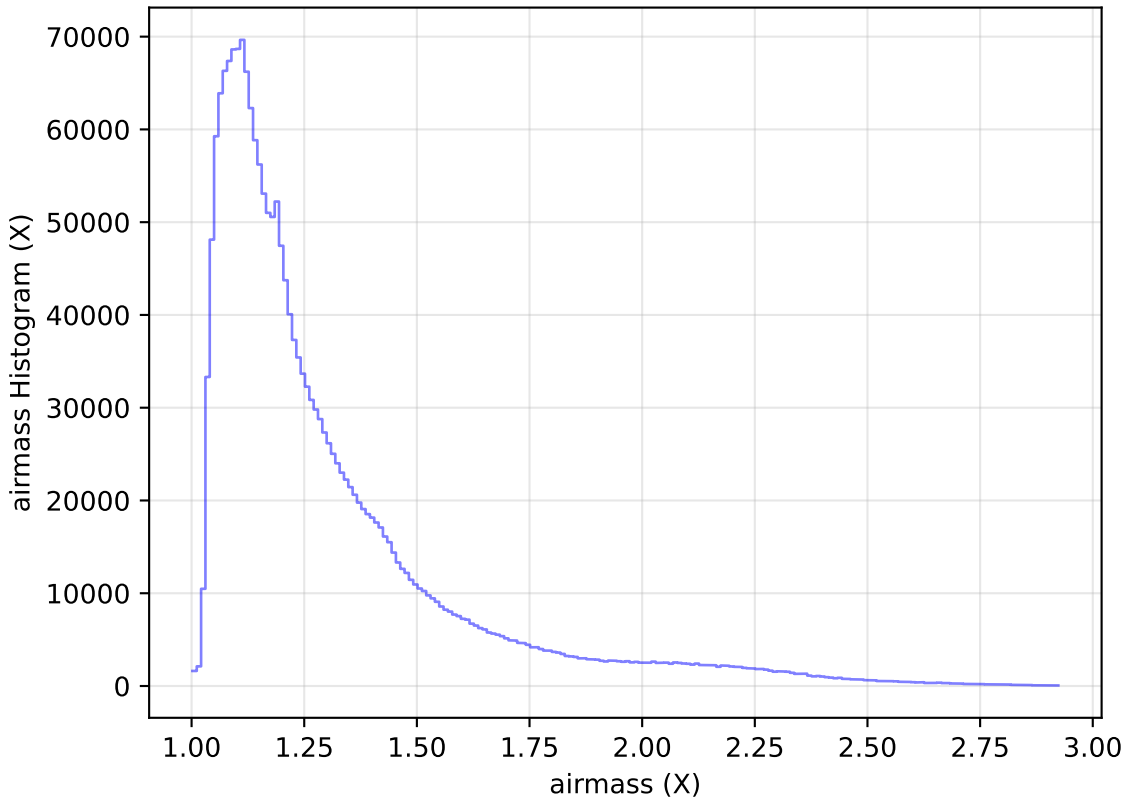
too_elab_r64_d3_giz_v3.4_10yrs All sky all bands: airmass Histogram
