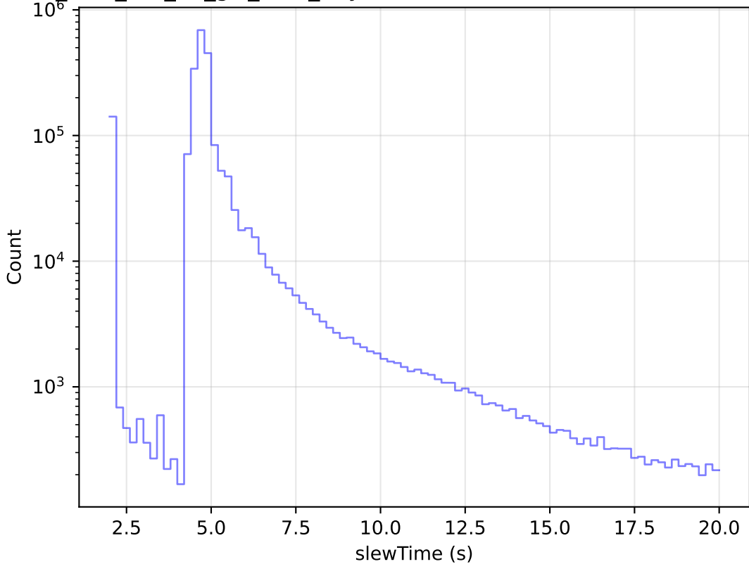
too_elab_r64_d3_giz_v3.4_10yrs All visits: Zoom Slew Time Histogram
