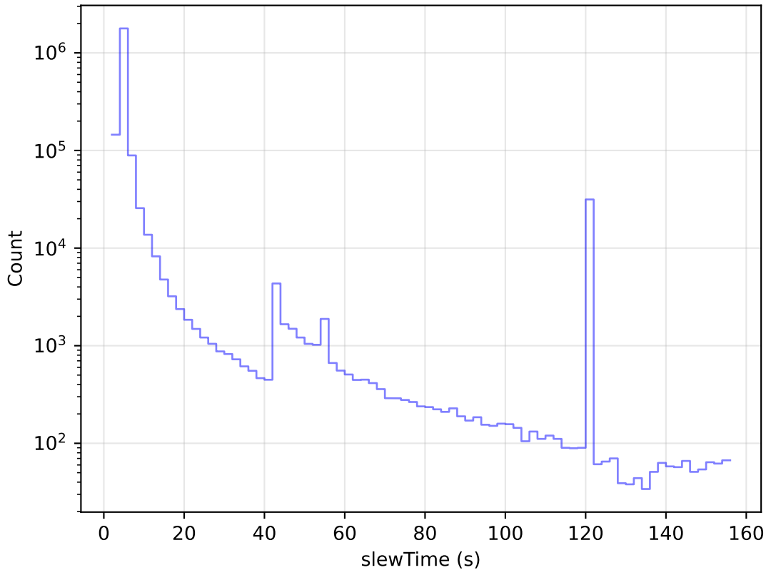
too_elab_r64_d3_giz_v3.4_10yrs All visits: Slew Time Histogram
