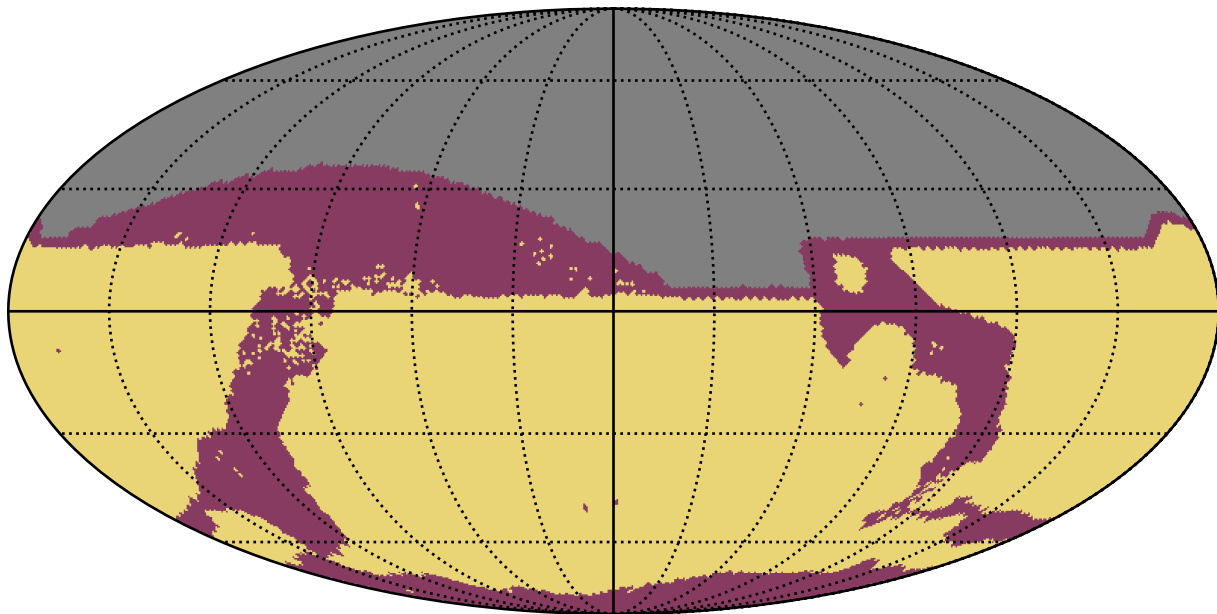
too_elab_r64_d3_giz_v3.4_10yrs All sky: RapidRevisits
