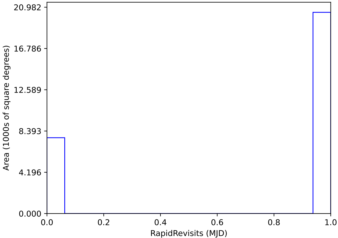
too_elab_r64_d3_giz_v3.4_10yrs All sky: RapidRevisits
