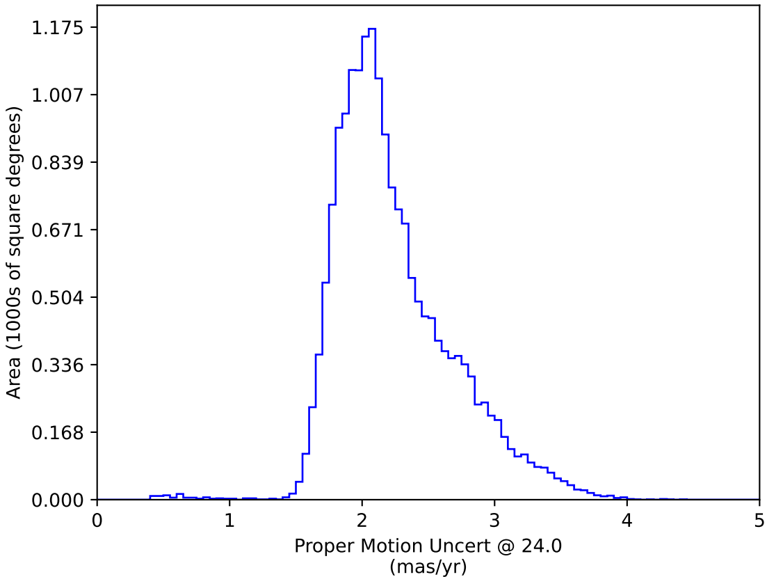
too_elab_r64_d3_giz_v3.4_10yrs WFD: Proper Motion Uncert @ 24.0
