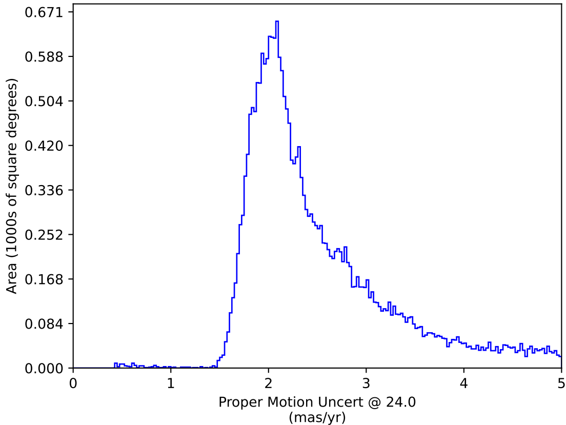
too_elab_r64_d3_giz_v3.4_10yrs All sky: Proper Motion Uncert @ 24.0
