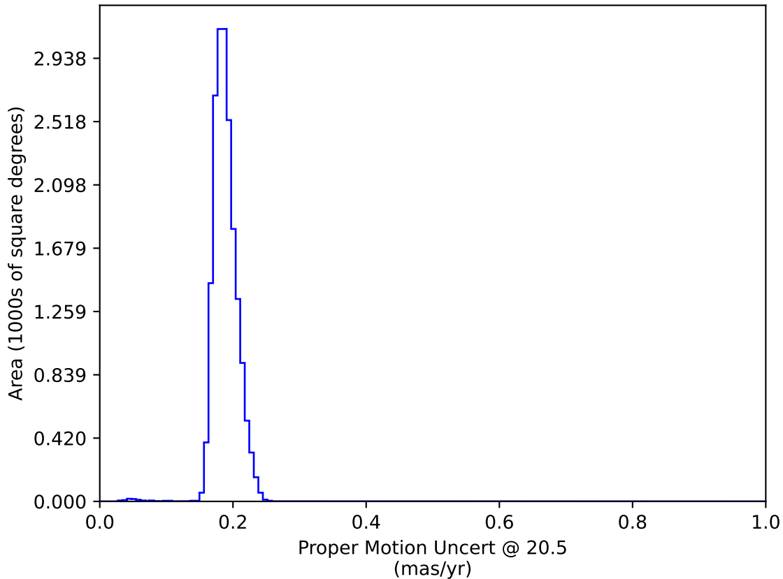
too_elab_r64_d3_giz_v3.4_10yrs WFD: Proper Motion Uncert @ 20.5
