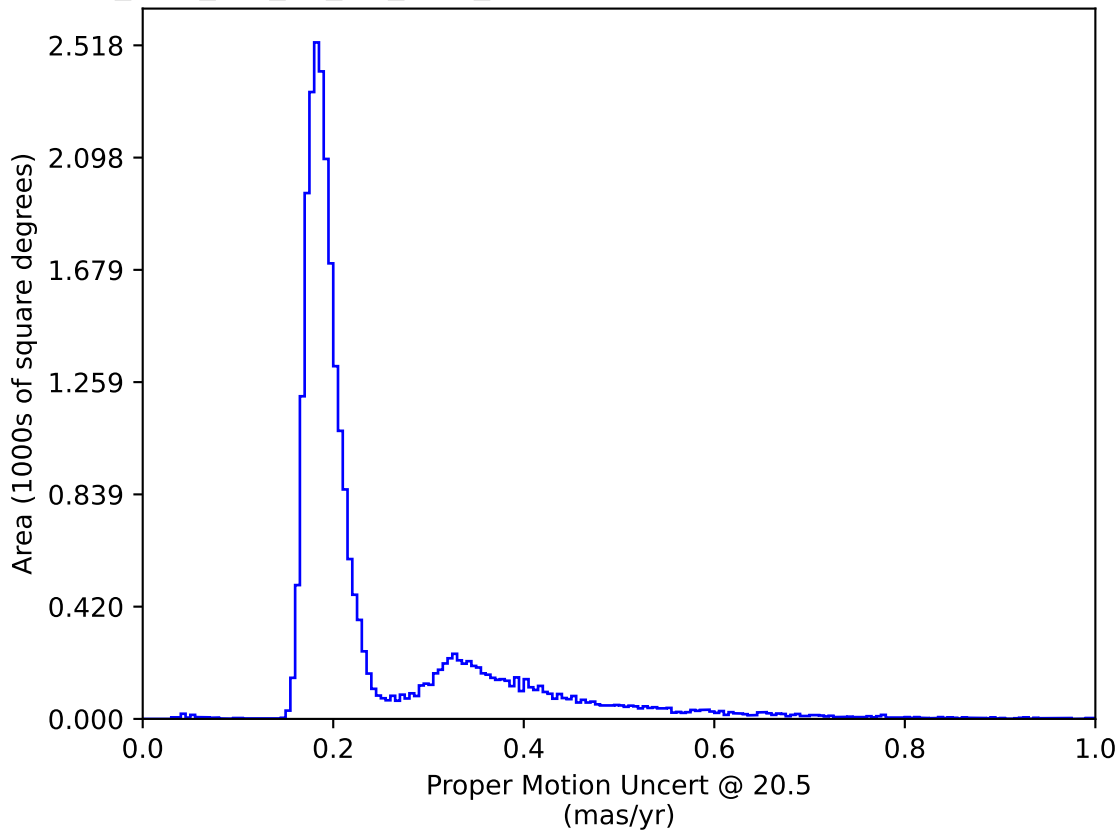
too_elab_r64_d3_giz_v3.4_10yrs All sky: Proper Motion Uncert @ 20.5
