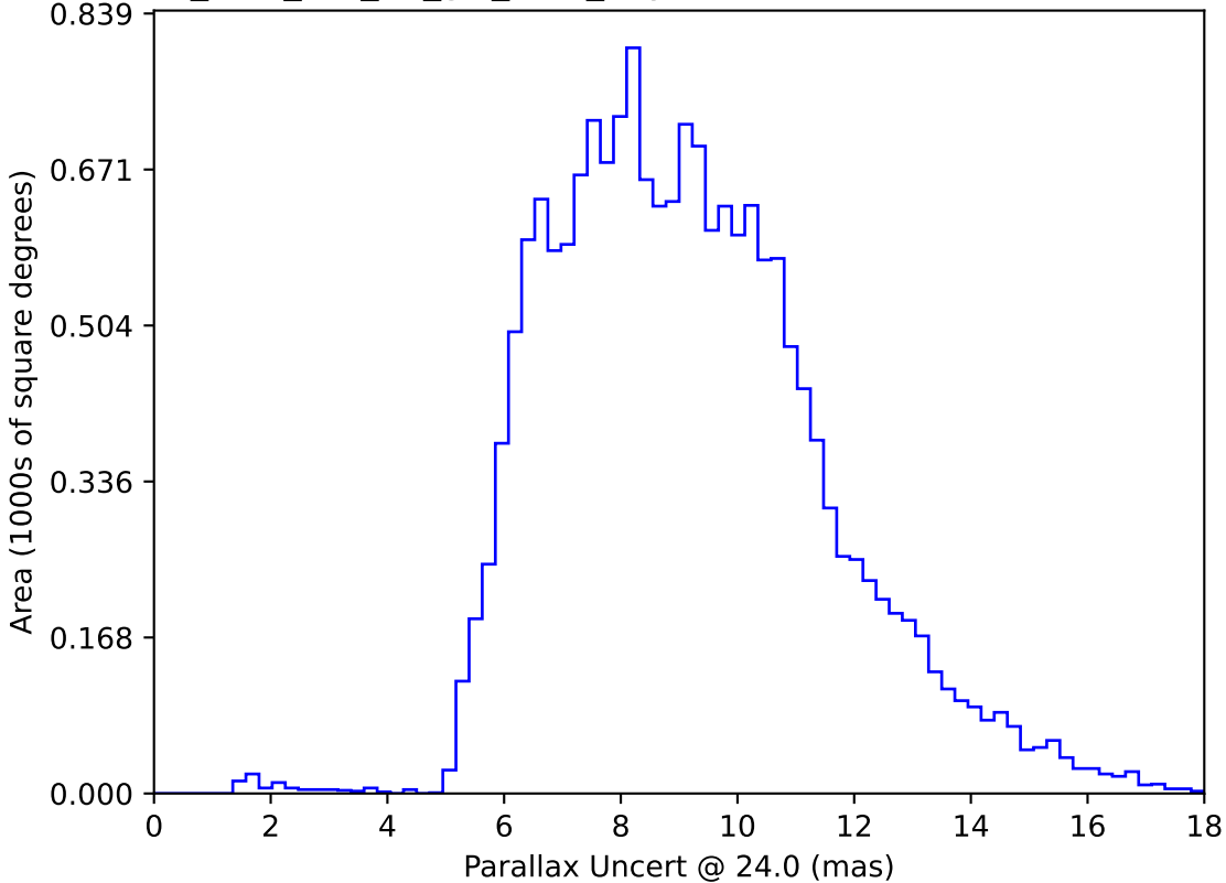
too_elab_r64_d3_giz_v3.4_10yrs WFD: Parallax Uncert @ 24.0
