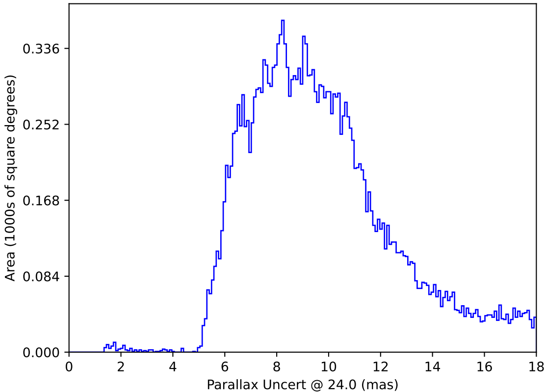
too_elab_r64_d3_giz_v3.4_10yrs All sky: Parallax Uncert @ 24.0
