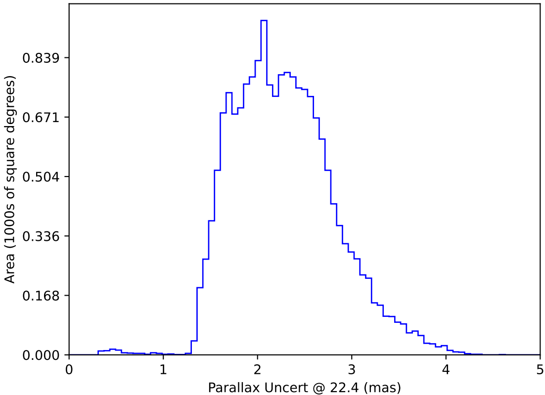
too_elab_r64_d3_giz_v3.4_10yrs WFD: Parallax Uncert @ 22.4
