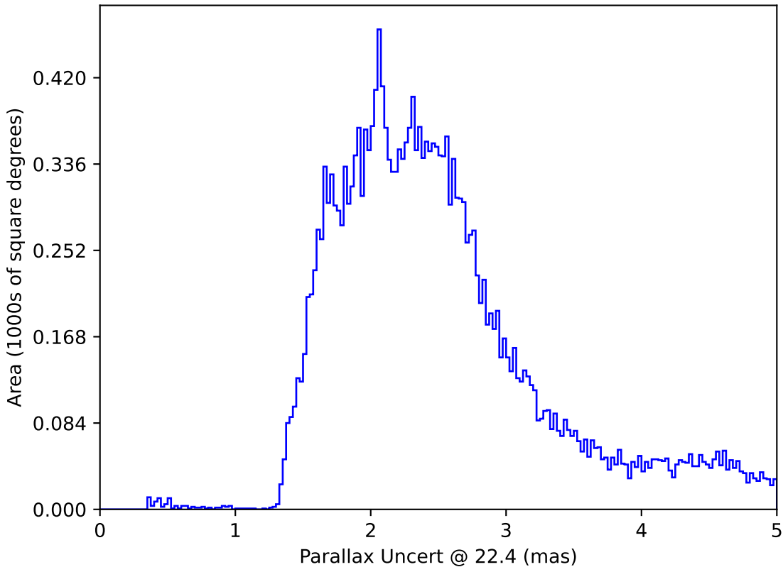
too_elab_r64_d3_giz_v3.4_10yrs All sky: Parallax Uncert @ 22.4
