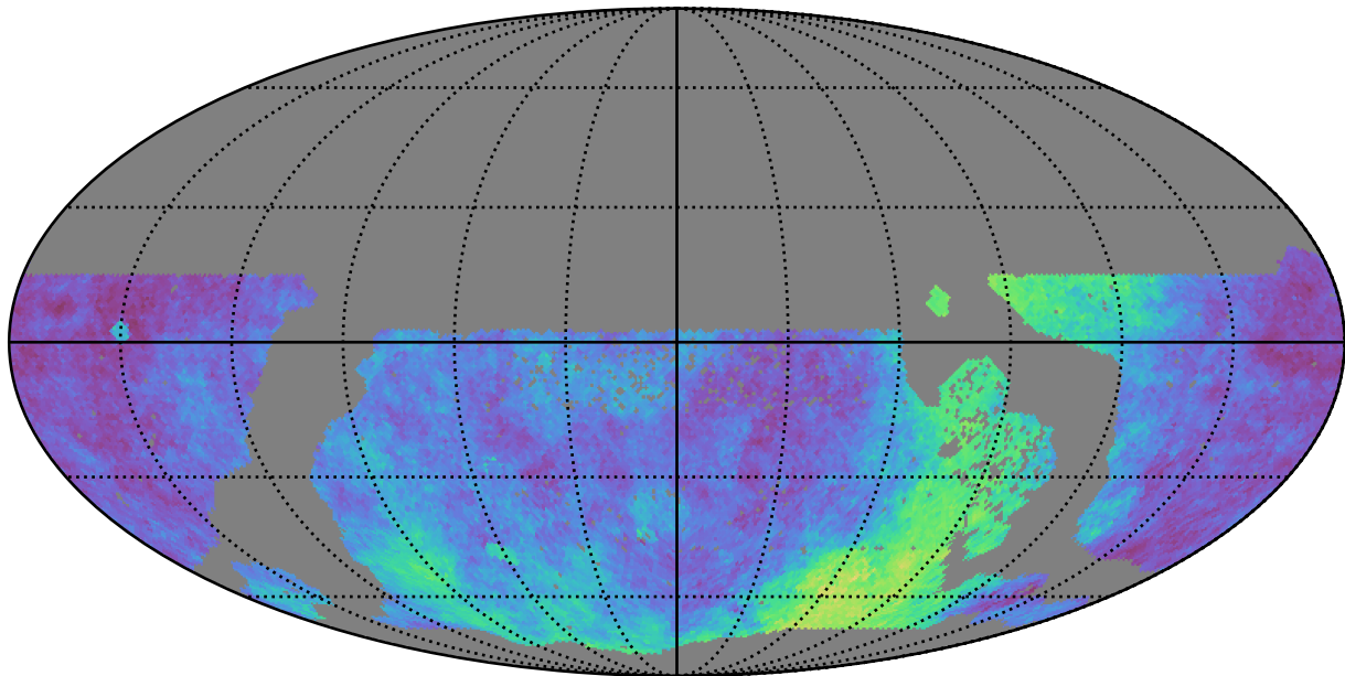
too_elab_r64_d3_giz_v3.4_10yrs WFD: Parallax Coverage @ 24.0
