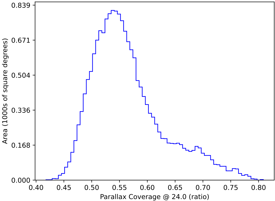
too_elab_r64_d3_giz_v3.4_10yrs WFD: Parallax Coverage @ 24.0
