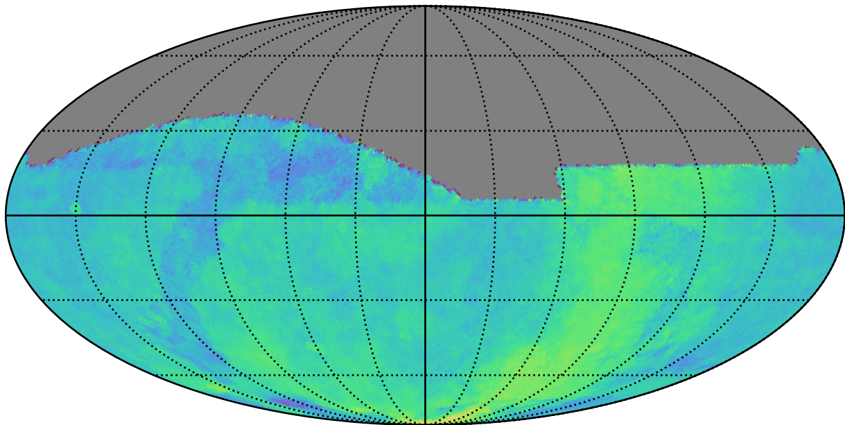
too_elab_r64_d3_giz_v3.4_10yrs All sky: Parallax Coverage @ 24.0
