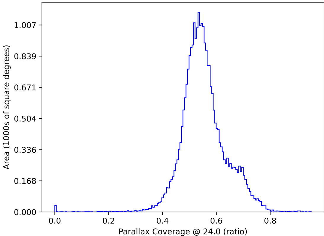
too_elab_r64_d3_giz_v3.4_10yrs All sky: Parallax Coverage @ 24.0
