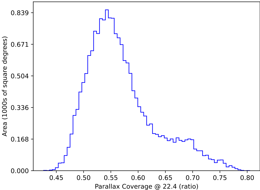
too_elab_r64_d3_giz_v3.4_10yrs WFD: Parallax Coverage @ 22.4
