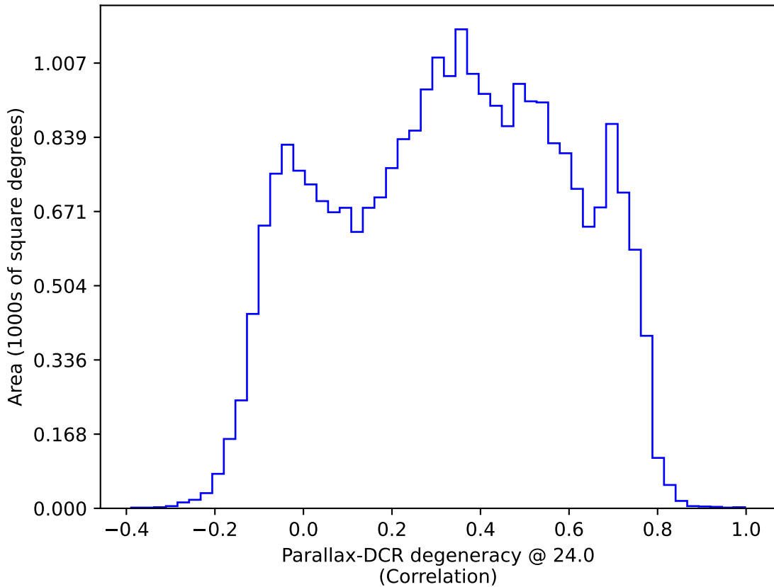
too_elab_r64_d3_giz_v3.4_10yrs All sky: Parallax-DCR degeneracy @ 24.0
