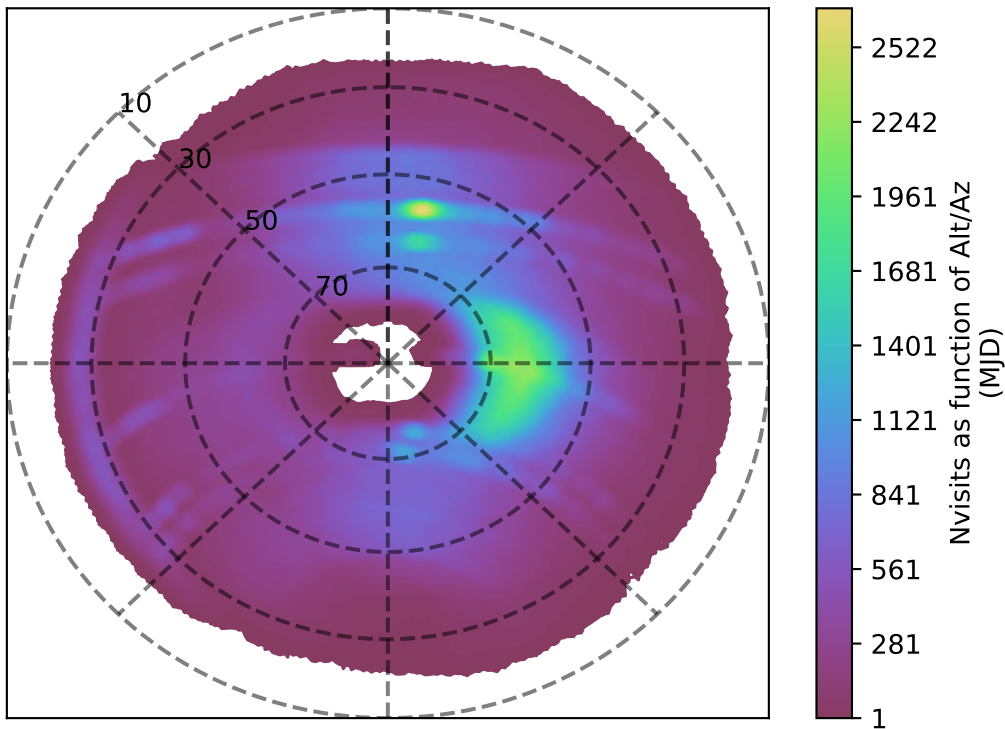
too_elab_r64_d3_giz_v3.4_10yrs r band: Nvisits as function of Alt/Az
