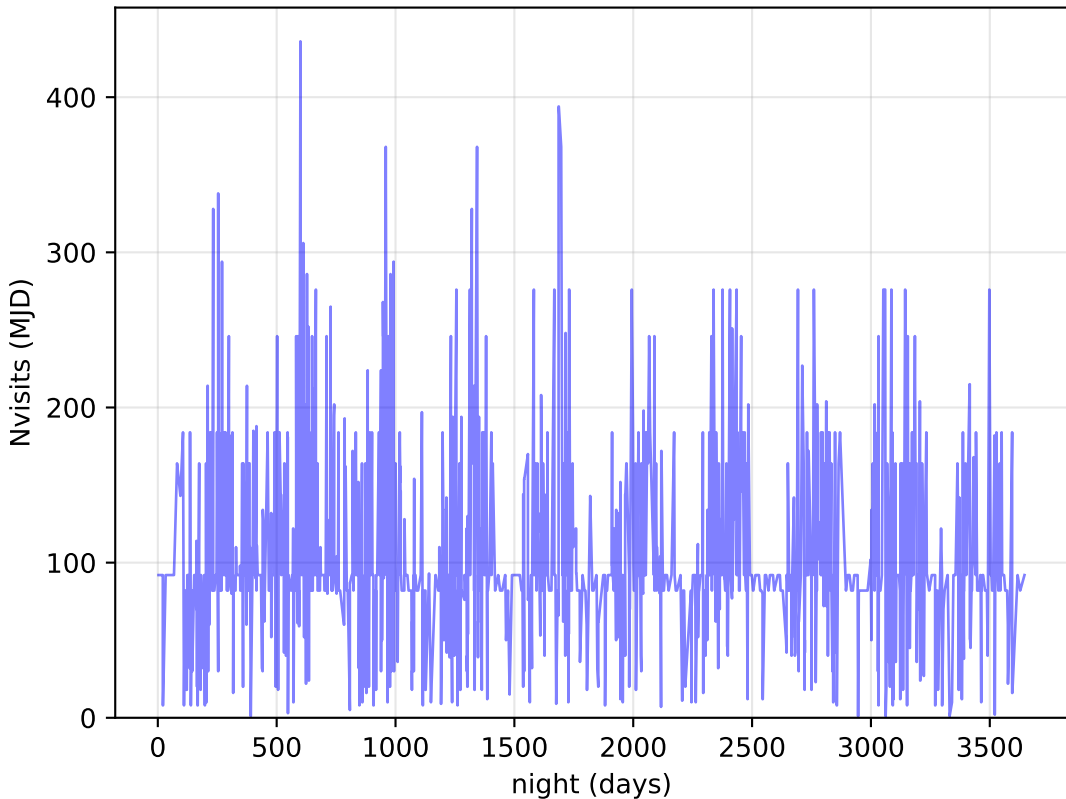
too_elab_r64_d3_giz_v3.4_10yrs DDF: Nvisits
