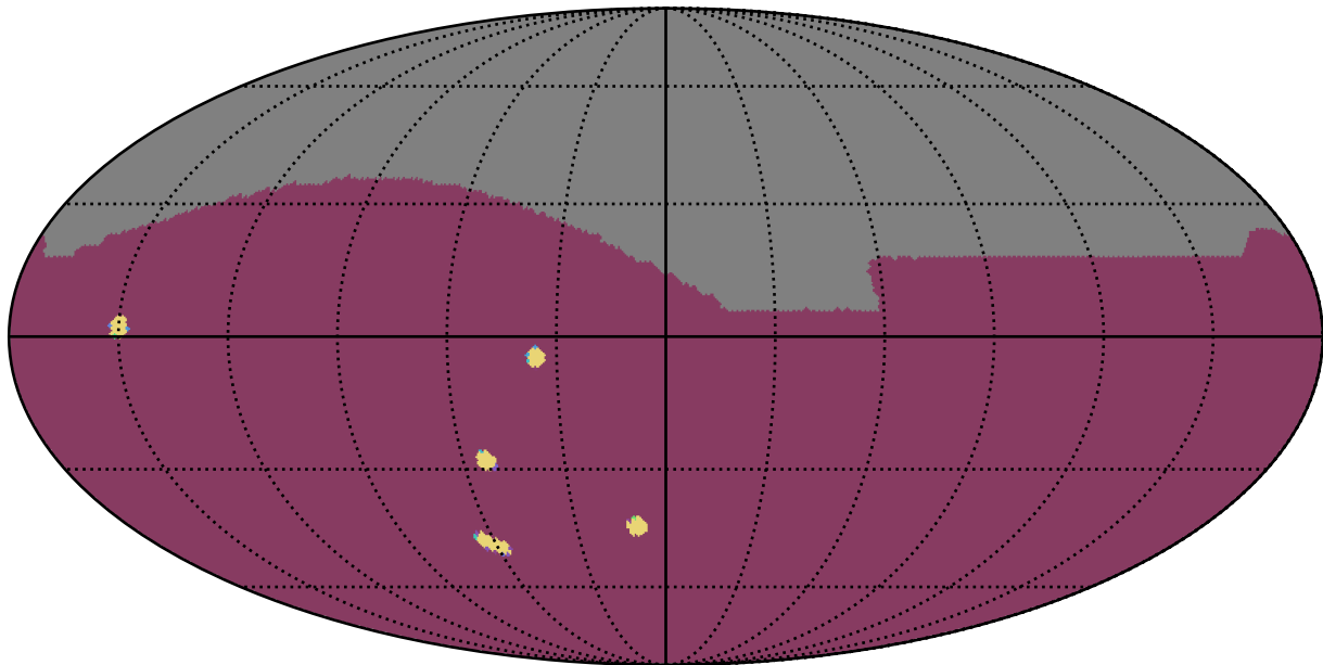
too_elab_r64_d3_giz_v3.4_10yrs All sky: NumberOfQuickRevisits
