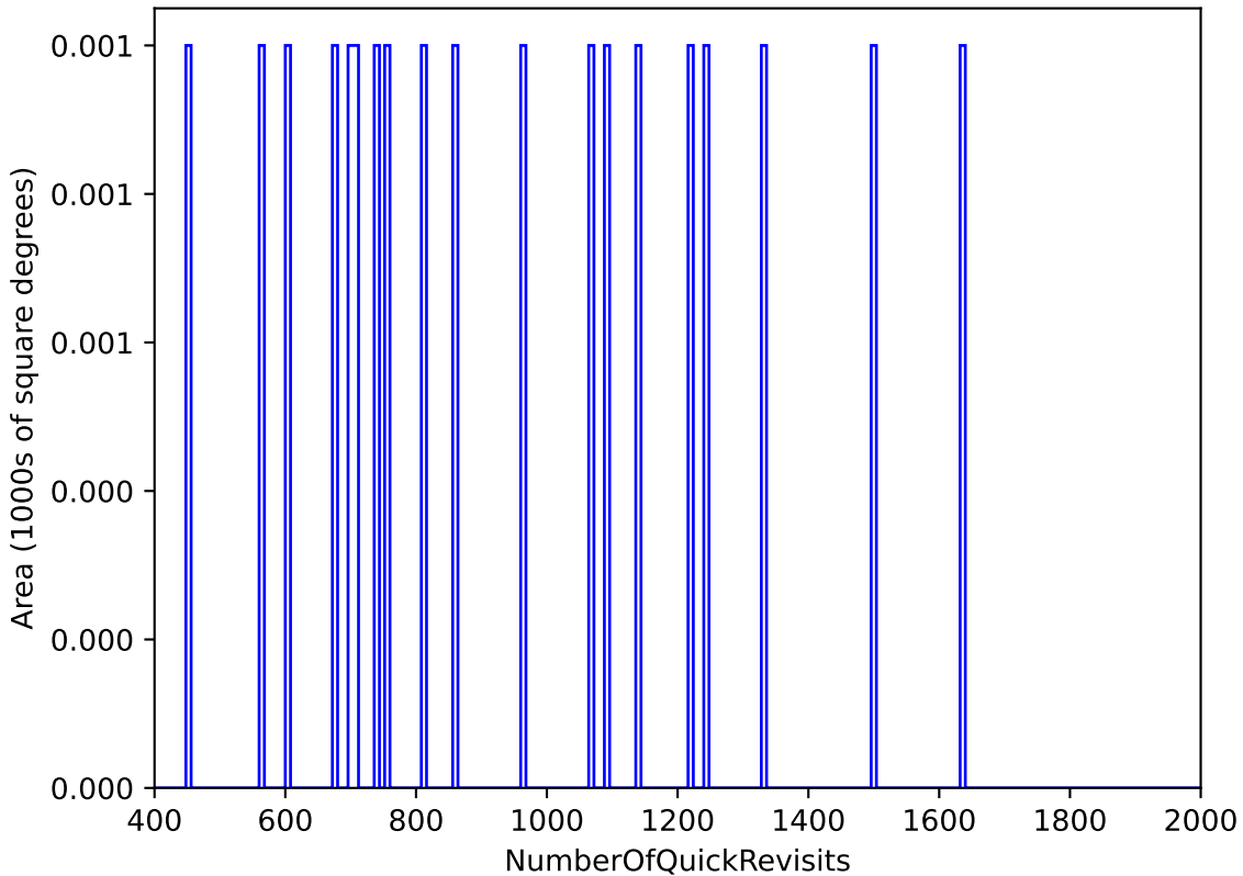
too_elab_r64_d3_giz_v3.4_10yrs All sky: NumberOfQuickRevisits
